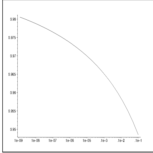
FIG. 4. Convergence rate estimate for the error norm of \varepsilon_h in W_2^4(\mathbb{R}^2) approximating the Laplacian on 6 general points by a stencil of polynomial exactness of order 3
