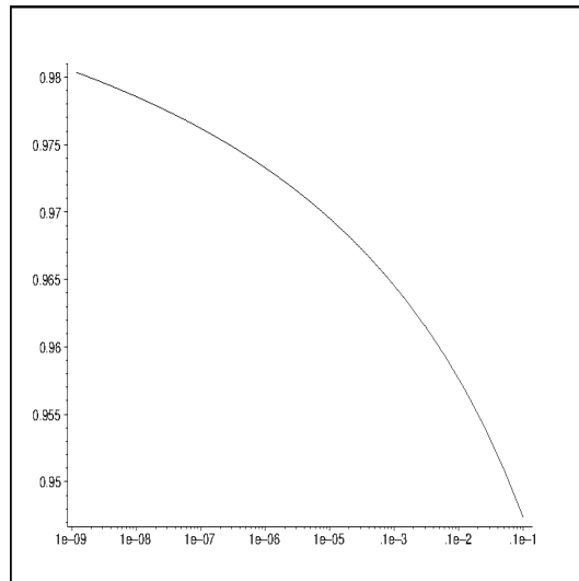
FIG. 2. Convergence rate estimates of the optimal \varepsilon_h in W_2^{4.5}(\mathbb{R}^3) approximating the Laplacian on 10 general points as function of h
