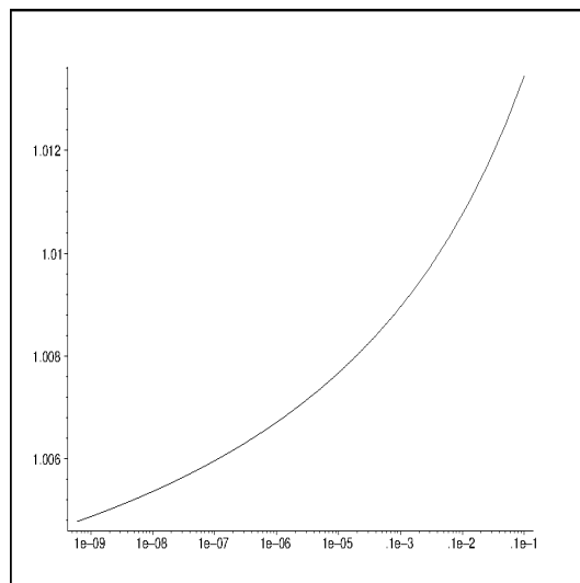
FIG. 3. Quotient between errors of polyharmonic and optimal Sobolev approximations as functions of h
