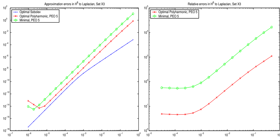
FIG. 11. Absolute and Sobolev-relative error norms in W_2^6(\mathbb{R}^2) for polyharmonic and minimal approximation of order 5 on set X3
