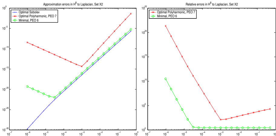
FIG. 8. Absolute and Sobolev-relative error norms in W_2^8(\mathbb{R}^2) for polyharmonic approximation of order 7 and minimal approximation of order 6 on set X2
