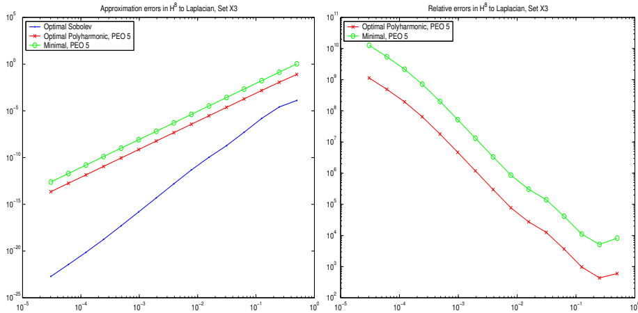
FIG. 10. Absolute and Sobolev-relative error norms in W_2^8(\mathbb{R}^2) for polyharmonic and minimal approximation of order 5 on set X3
