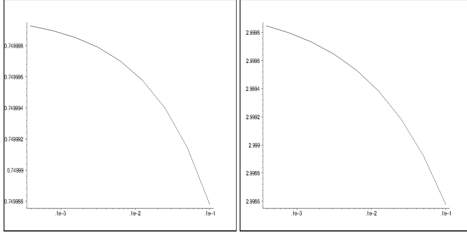
FIG. 1. Convergence rate estimates of the optimal \varepsilon_h in W_2^{3.75}(\mathbb{R}^2) and W_2^{6.25}(\mathbb{R}^2) approximating the Laplacian on 18 general points as function of h
