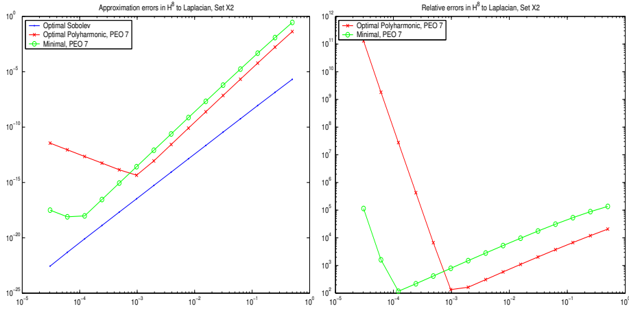
FIG. 6. Absolute and Sobolev-relative error norms in W_2^8(\mathbb{R}^2) for approximations with polynomial exactness order (PEO) 7 on set X2
