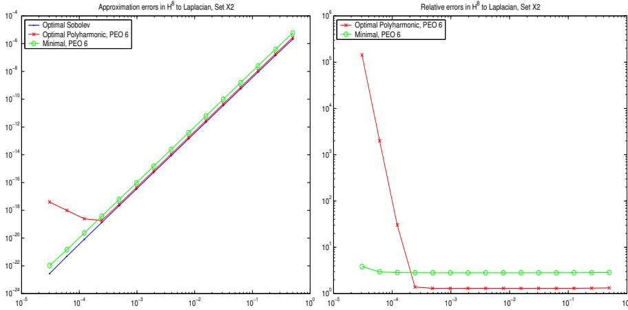
FIG. 7. Absolute and Sobolev-relative error norms in W_2^8(\mathbb{R}^2) for approximations with polynomial exactness order 6 on set X2
