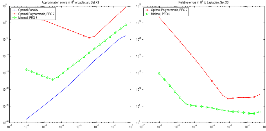
FIG. 9. Absolute and Sobolev-relative error norms in W_2^8(\mathbb{R}^2) for polyharmonic approximation of order 7 and minimal approximation of order 6 on set X3
