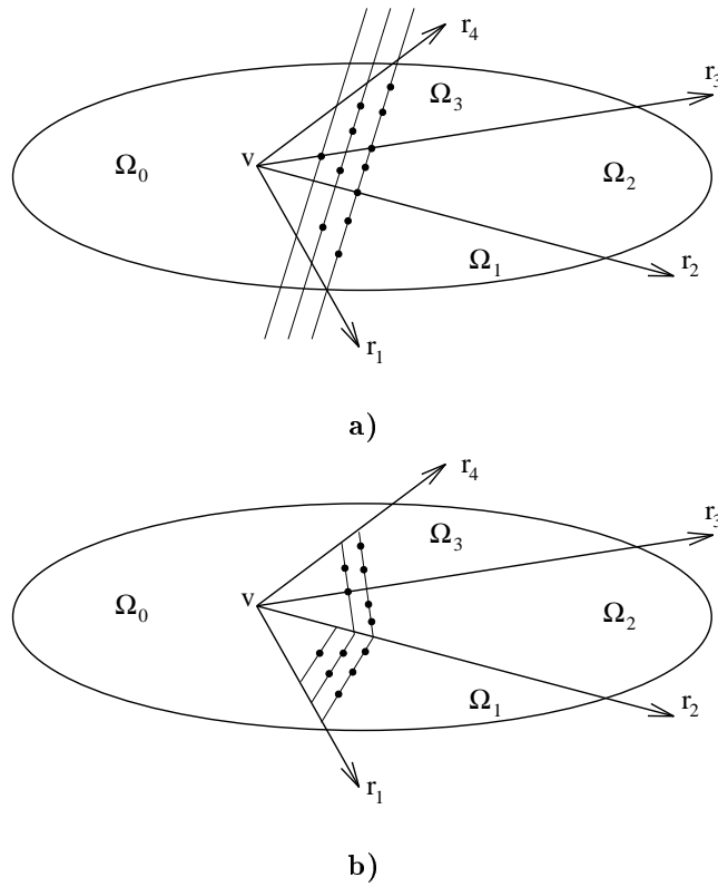
Fig. 2.4. Interpolation points of type C.
