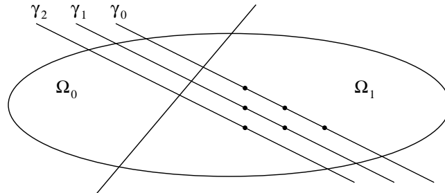
Fig. 2.2. Interpolation points of type B.
