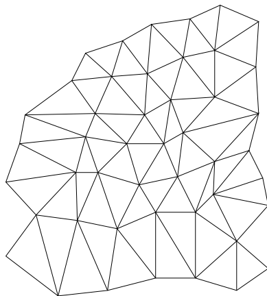
Fig. 3.4. An example of partition \tilde{\Delta}^1 .
