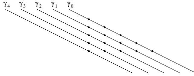
Fig. 2.1. Interpolation points of type A.
